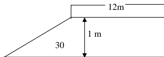
Diagram 2. Competition Platform
